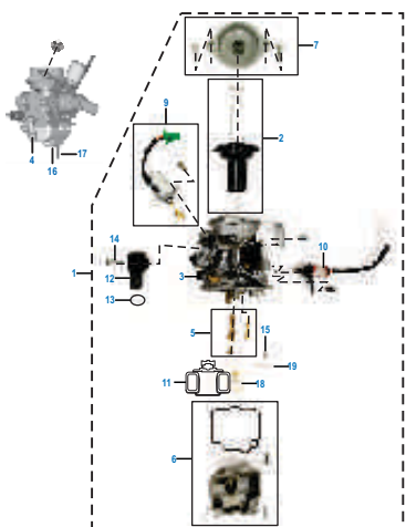
PLATE NO. : 18 CARBURETTOR
