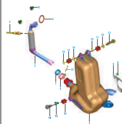
PLATE NO. : 21 SILENCER ASSEMBLY
