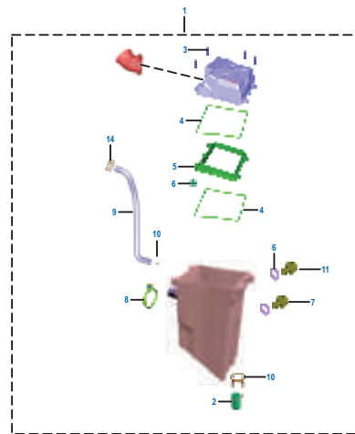
PLATE NO. : 19 AIR CLEANER COMPLETE - FI VERSION
