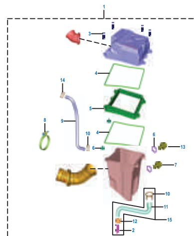
PLATE NO. : 19A AIR CLEANER COMPLETE
