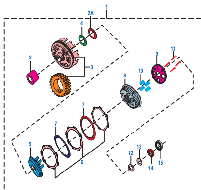
PLATE NO.: 16 CLUTCH ASSEMBLY
