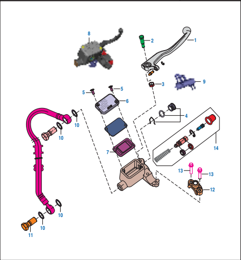
PLATE NO. : 35 FRONT MASTER CYLINDER - DISC BRAKE
