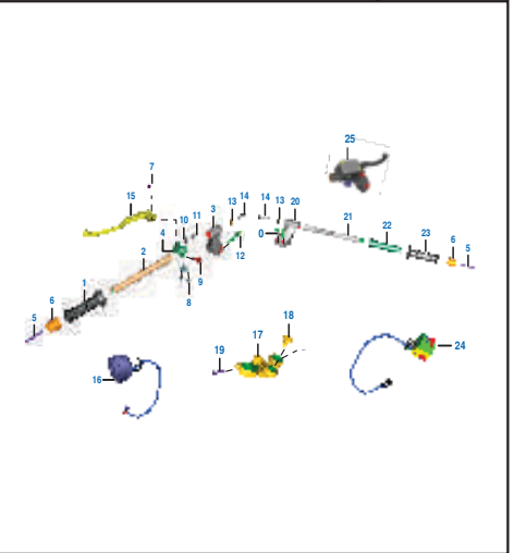
PLATE NO. : 40 HANDLE BAR ASSEMBLY
