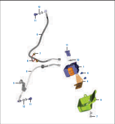
PLATE NO. : 39 ANTI LOCK BRAKING SYSTEM
