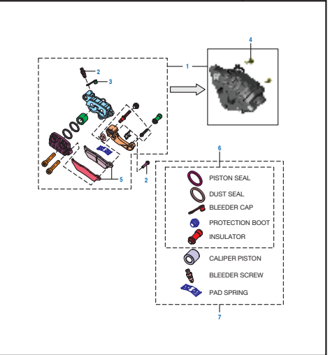
PLATE NO. : 36 FRONT CALIPER ASSEMBLY - DISC BRAKE
