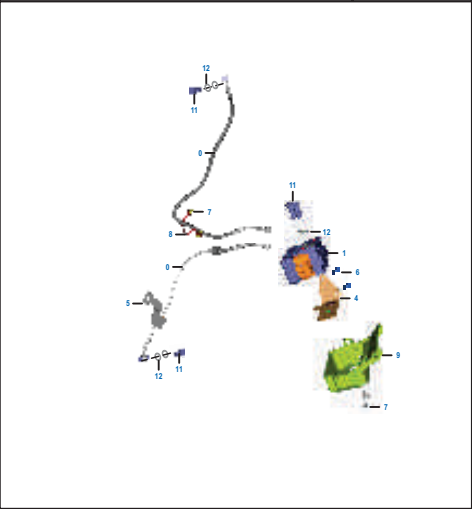
PLATE NO. : 37 ANTILOCK BRAKING SYSTEM PAGE NO. 83
