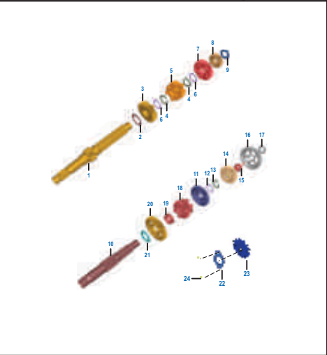
PLATE NO. : 7 TRANSMISSION
