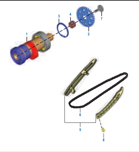
PLATE NO. : 4 CAMSHAFT
