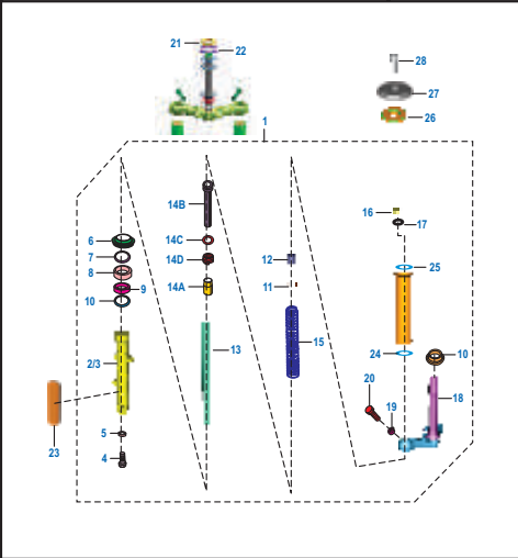
PLATE NO. : 40 FRONT FORK PAGE NO. 99 - 95
