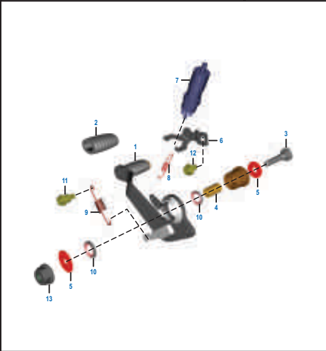
PLATE NO. : 36 REAR BRAKE PEDAL PAGE NO. 81
