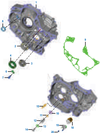
PLATE NO. : 11 CRANKCASE RH
