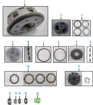
PLATE NO. : 16 CLUTCH ASSEMBLY
