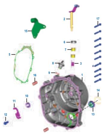
PLATE NO. : 14 COVER CLUTCH
