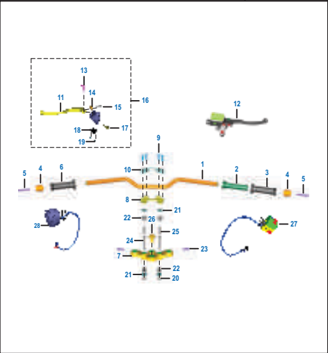
PLATE NO. : 39 HANDLEBAR ASSEMBLY - N250 PAGE NO. 89 - 91
