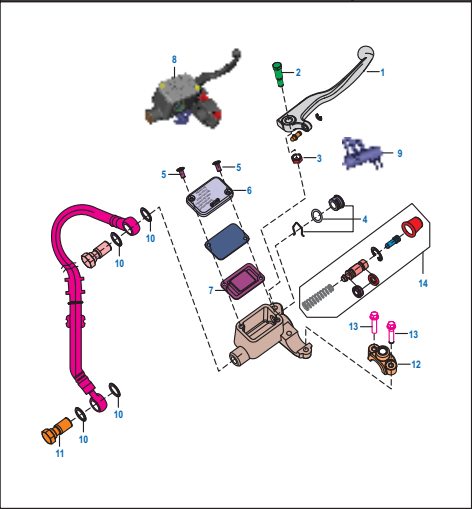
PLATE NO. : 33 FRONT MASTER CYLINDER - DISC BRAKE PAGE NO. 75
