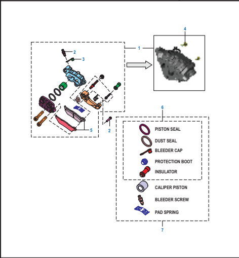
PLATE NO. : 34 FRONT CALIPER ASSEMBLY - DISC BRAKE PAGE NO. 77
