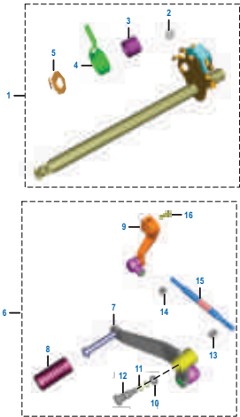
PLATE NO. : 9 GEAR CHANGE MECHANISM
