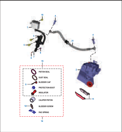
PLATE NO. : 35 REAR DISC BRAKE ASSEMBLY PAGE NO. 79
