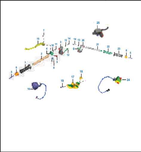
PLATE NO. : 38 HANDLEBAR ASSEMBLY - F250 PAGE NO. 85 - 87
