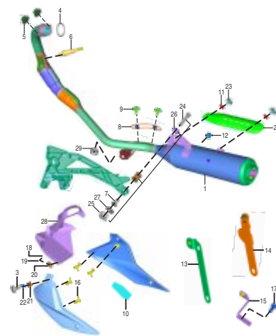
PLATE NO. : 18 SILENCER ASSEMBLY & BELLY PAN
