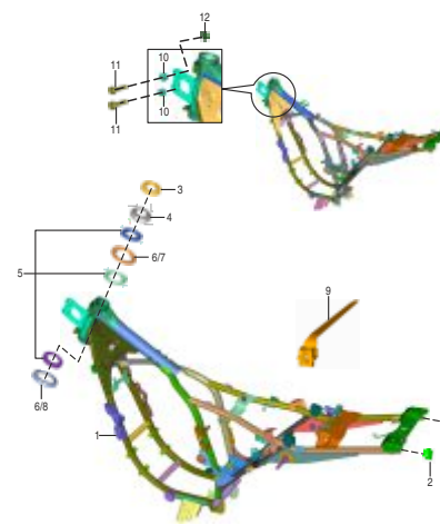
PLATE NO. : 23 FRAME AND FRAME FITTINGS
