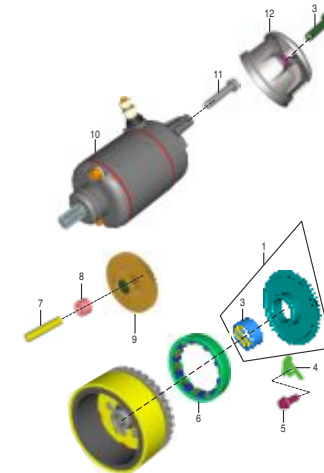
PLATE NO. : 22 STARTER ASSEMBLY
