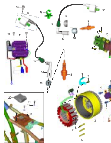
PLATE NO. : 21 MAGNETO, ECU & H.T. COIL
