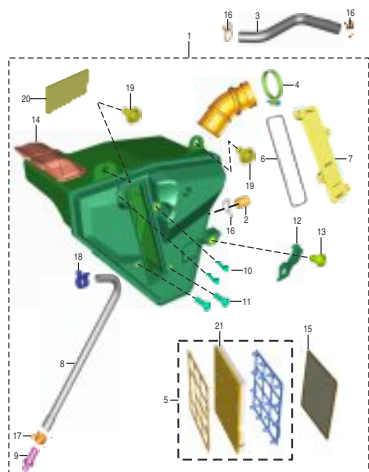
PLATE NO. : 19 AIR CLEANER ASSEMBLY
