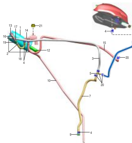
PLATE NO. : 20 EVAP MECHANISM
