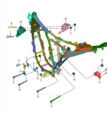
PLATE NO. : 24 ENGINE MOUNTINGS
