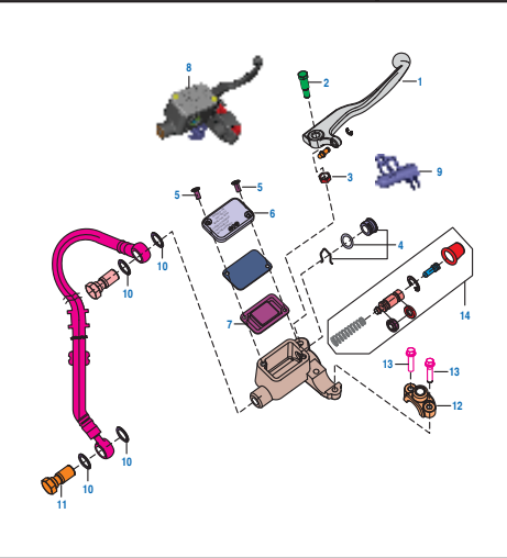
PLATE NO. : 36 FRONT MASTER CYLINDER - DISC BRAKE
