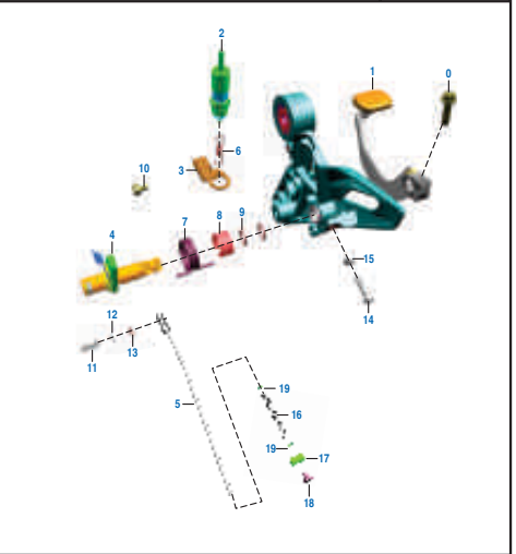
PLATE NO. : 39 REAR BRAKE PEDAL - DRUM BRAKE
