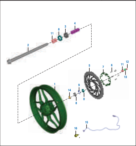
PLATE NO. : 33 FRONT WHEEL HUB
