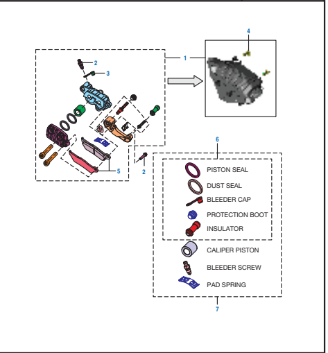
PLATE NO. : 37 FRONT CALIPER ASSEMBLY - DISC BRAKE
