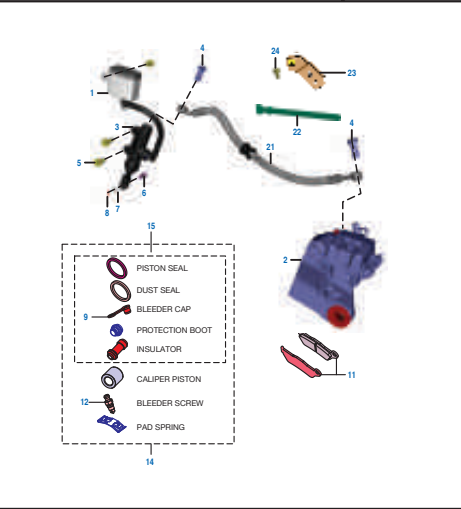
PLATE NO. : 40 REAR BRAKE PEDAL - REAR DISC BRAKE (TWIN DISC)
