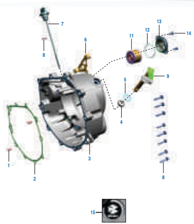
PLATE NO. : 15 KICK STARTER MECHANISM
