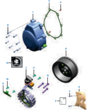
PLATE NO. : 14 COVER MAGNETO
