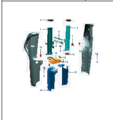
PLATE NO. : 48 FORK COVER ASSEMBLY-DISC/DRUM LED
