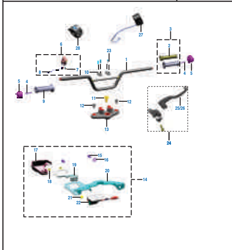
PLATE NO. : 42 HANDLE BAR ASSEMBLY
