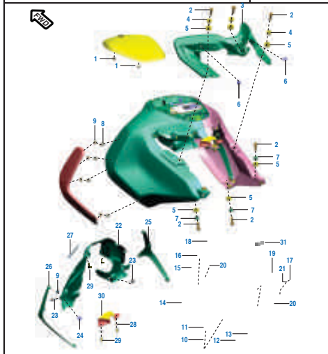
PLATE NO. : 44 ASSEMBLY TANK COVER
