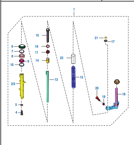
PLATE NO. : 43 FRONT FORK
