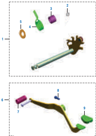
PLATE NO. : 11 CRANKCASE RH
