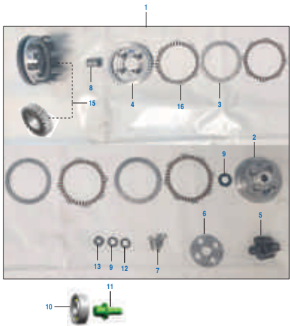
PLATE NO. : 16 / 16A CLUTCH ASSEMBLY - ENDURANCE/MAKINO
