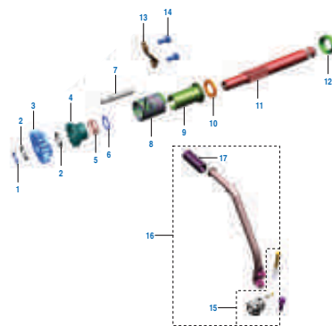
PLATE NO. : 15 KICK STARTER MECHANISM
