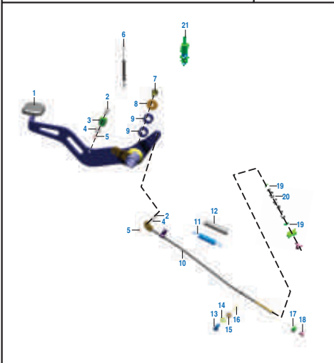
PLATE NO. : 41 REAR BRAKE PEDAL - DRUM BRAKE
